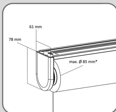
J41 & J51 (incl. steun)
