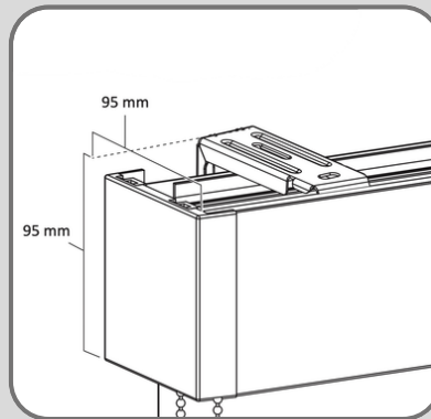
J42, J52, J43 & J53 (incl. steun)
