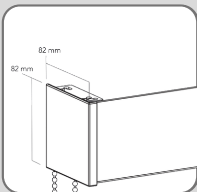
J45 & J55 (incl. steun)
